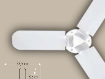
CT-1152 PERVANE AMPUL
